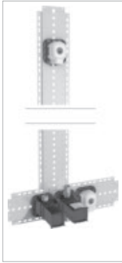
HANSAMATRIX installation unit set 04 thermostatic mixer, DN 15 (G1/2) 4486 0040 for two wall outlets suitable for trim kit installation set 08
