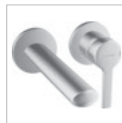
HANSARONDA trim kit wall-mounted single-lever basin mixer, DN 15* 0383 2273 chrome projection: 182 mm
