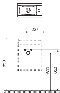
SD Classic 400 + Classic 400 L
