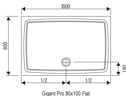
Gigant Pro 80x100 Flat
