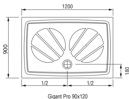
Gigant Pro 90x120
