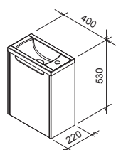
SD Classic 400 + Classic 400
