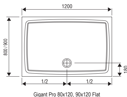
Gigant Pro 80x120, 90x120 Flat
