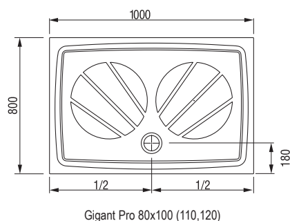
Gigant Pro 80x100 (110,120)
